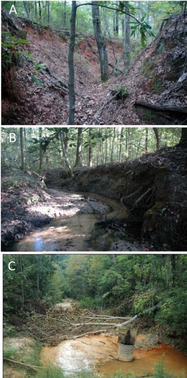
Figure 3. Turner Branch stabilized headwater gullies(A) and unstable perennial channel (B). Upper Three Runs tributary severely incised by runoff from an SRS industrial area (C).
