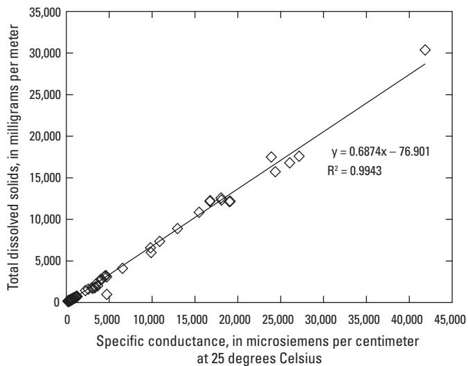
Figure 3. Correlation between total dissolved solids (TDS) and specific conductance using 139 water-quality samples from 40 wells in Chatham County, Georgia.
